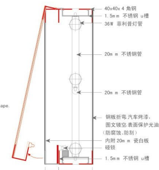
▲ 剖面图 (Cross-section)
